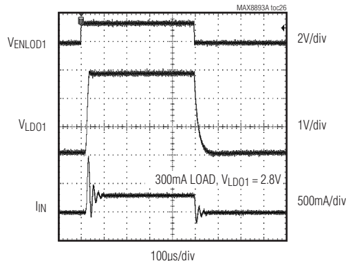
LD01 STARTUP AND SHUTDOWN WAVEFORM
