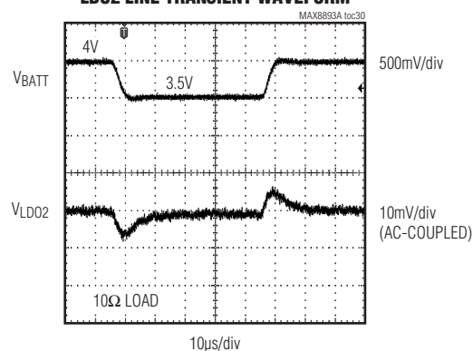
LD02 LINE TRANSIENT WAVEFORM
