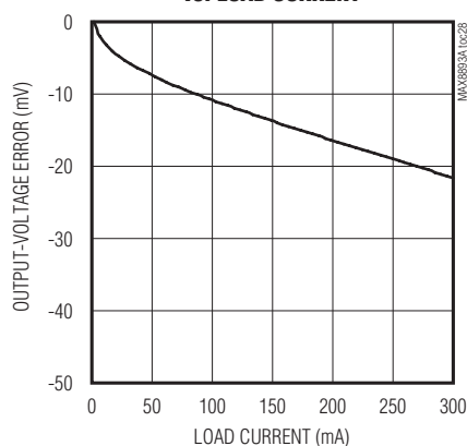
LD02 OUTPUT-VOLTAGE ERROR vs. LOAD CURRENT
