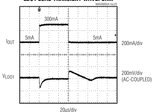
LD01 LOAD TRANSIENT WAVEFORM
