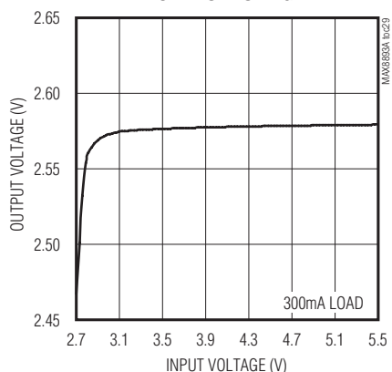
LD02 OUTPUT VOLTAGE vs. INPUT VOLTAGE
