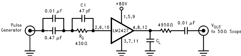
Typical Test Circuit (One Section)
