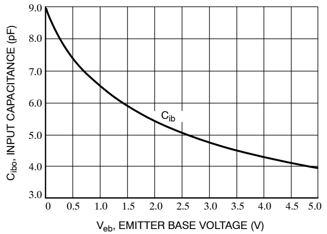
Figure 13. Input Capacitance
