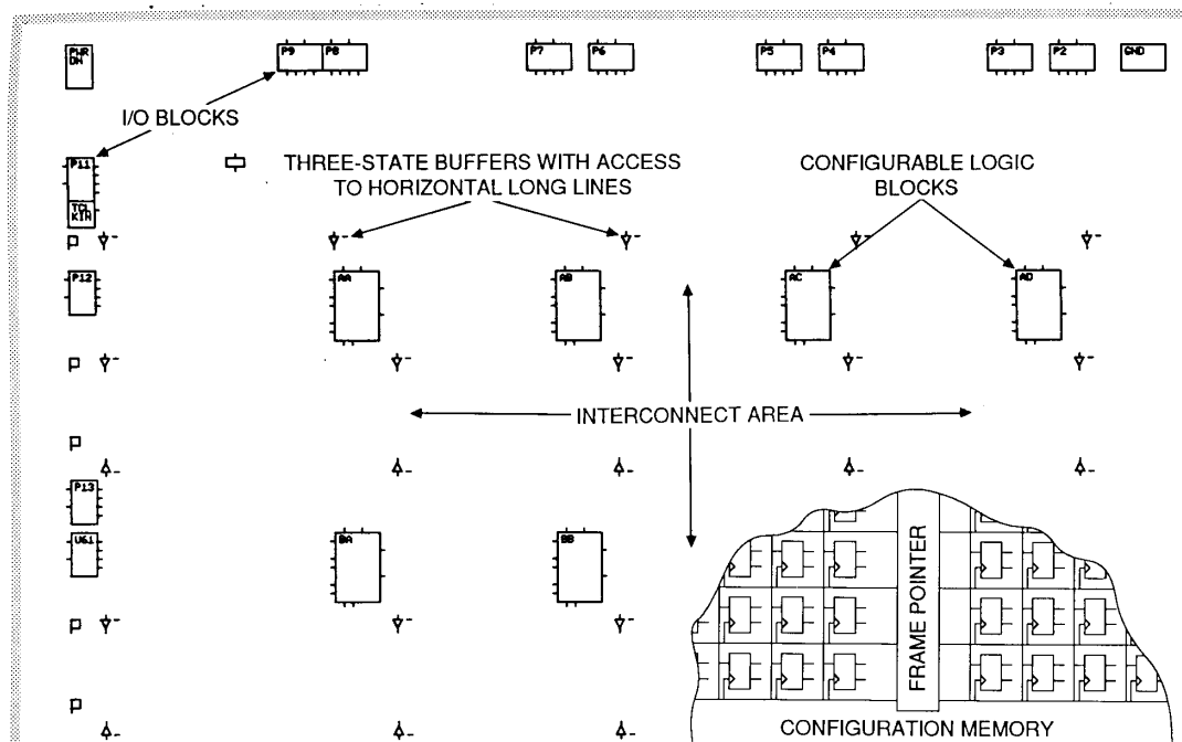
Figure 1. Field-Programmable Gate Array Structure
