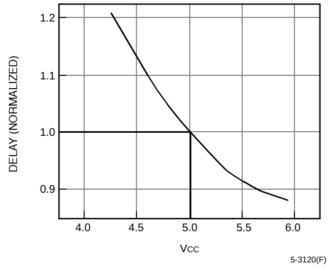
Figure 29. Speed Performance of a CMOS Device
