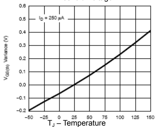
Threshold Voltage
