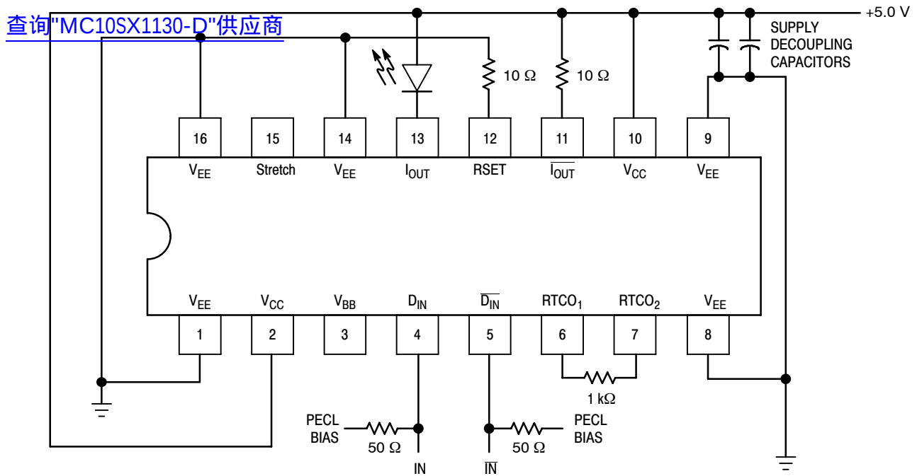
Figure 3. Typical +5 V Applications Circuit
