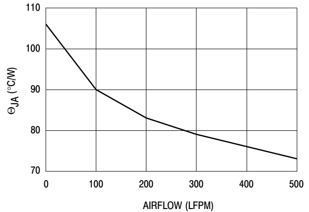
Figure 4. Typical \theta_{JA} versus Airflow
