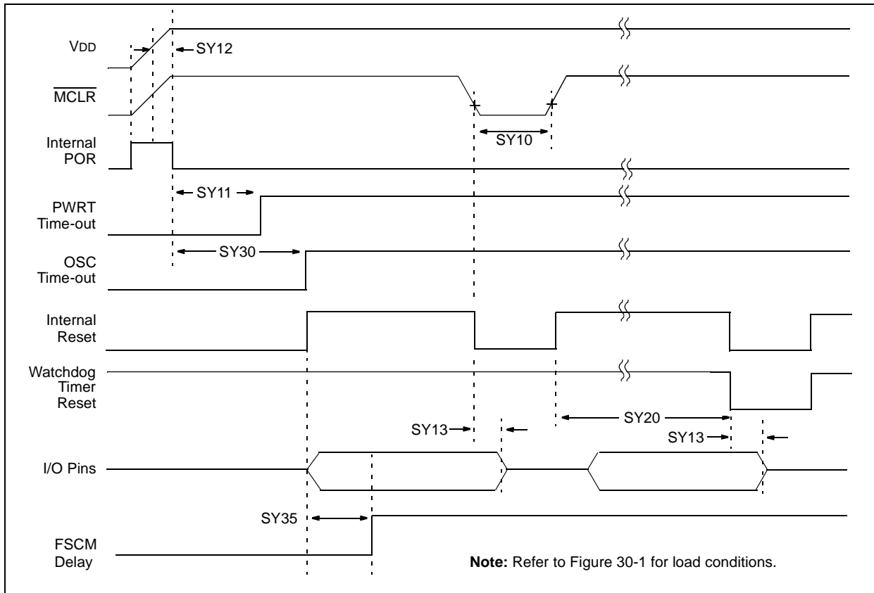
FIGURE 30-4: (RESET WATCHDOG TIMER, OSCILLATOR START-UP TIMER AND POWER-UP TIMER) TIMER TIMING CHARACTERISTICS
