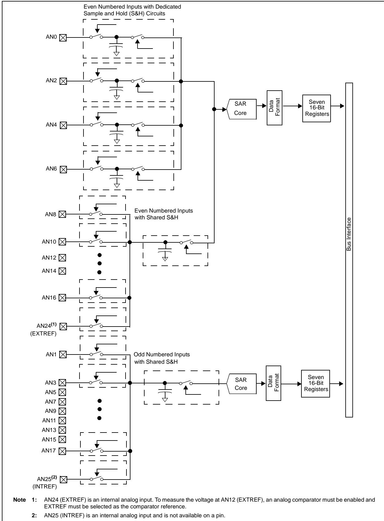
查询 FIGURE 22-36 dsPIC33FJ64GS406/606/608/610 ADC BLOCK DIAGRAM FOR dsPIC33FJ32GS608 AND dsPIC33FJ64GS608 DEVICES WITH TWO SARs
