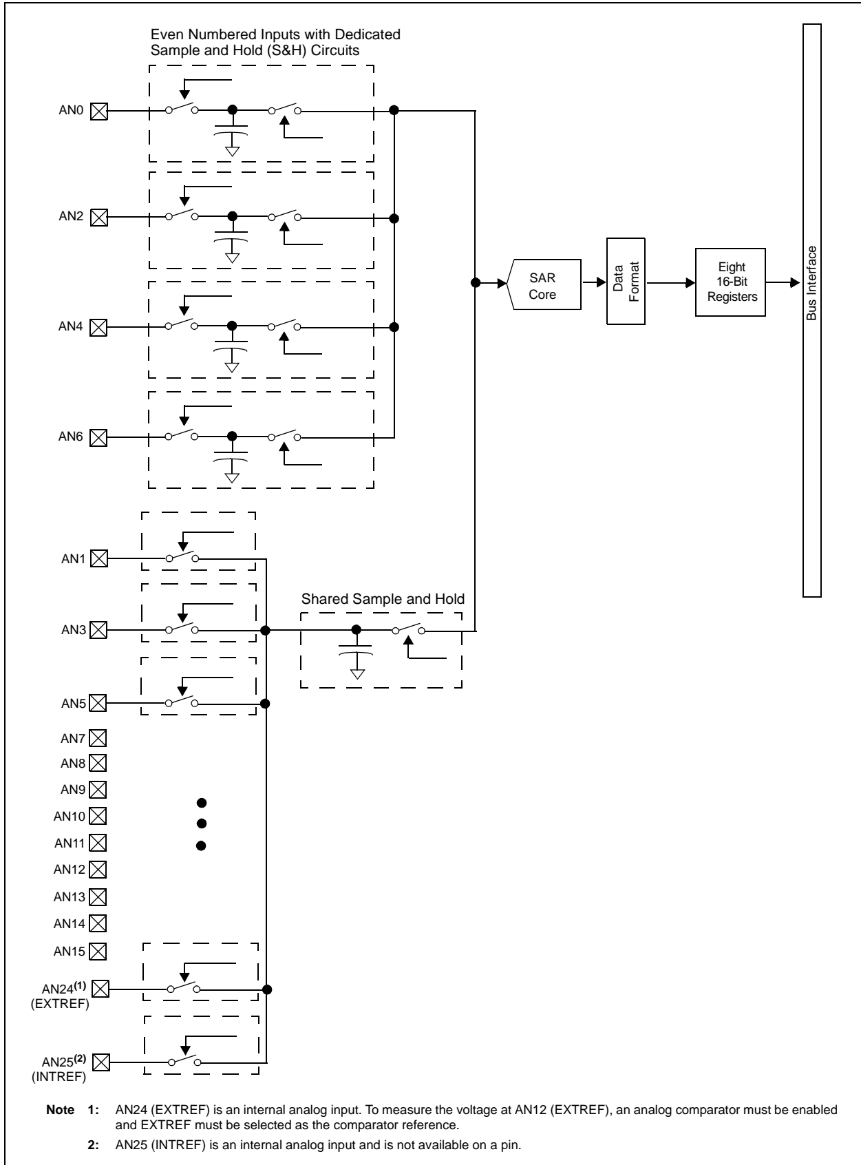
查询 FIGURE 22-16 dsPIC33FJ64GS406 数据手册 FIGURE 22-16 ADC BLOCK DIAGRAM FOR dsPIC33FJ32GS406 AND dsPIC33FJ64GS406 DEVICES WITH ONE SAR
