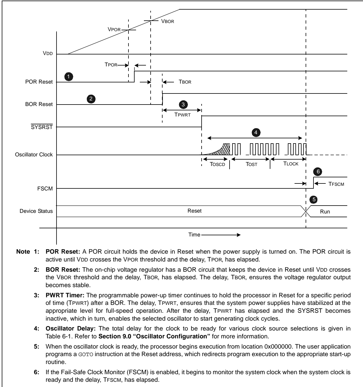
查询dsPIC33FJ64GS406供应商 FIGURE 6-2: SYSTEM RESET TIMING
