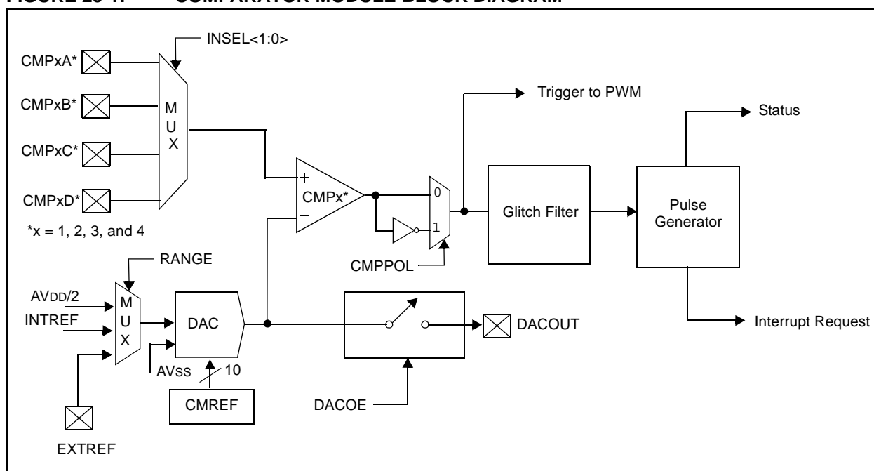
FIGURE 23-1: COMPARATOR MODULE BLOCK DIAGRAM
