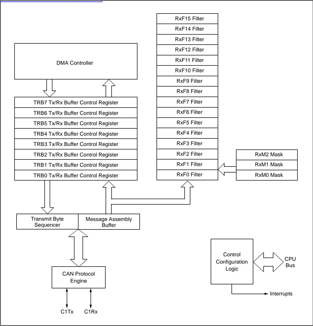
FIGURE 21-36 dsPIC33FJ64GS406/606/608/610 CAN™ MODULE BLOCK DIAGRAM
