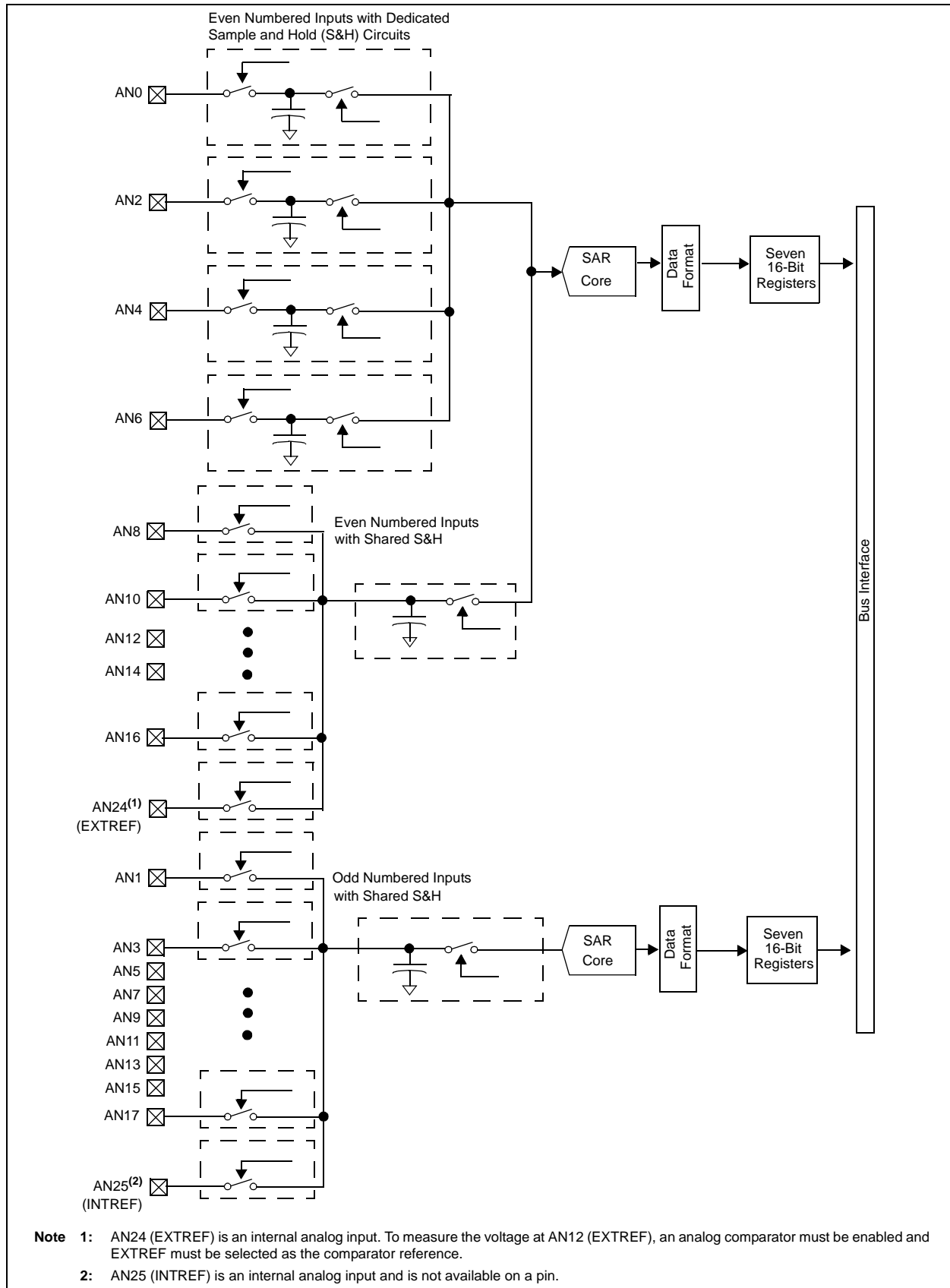
FIGURE 22-36 ADC BLOCK DIAGRAM FOR dsPIC33FJ32GS608 AND dsPIC33FJ64GS608 DEVICES WITH TWO SARs
