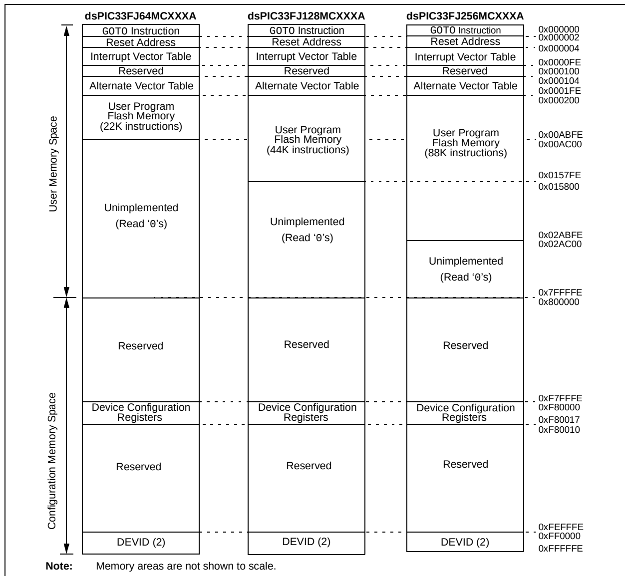
FIGURE 4-1: PROGRAM MEMORY MAP FOR dsPIC33FJXXMXX06A/X08A/X10A DEVICES
