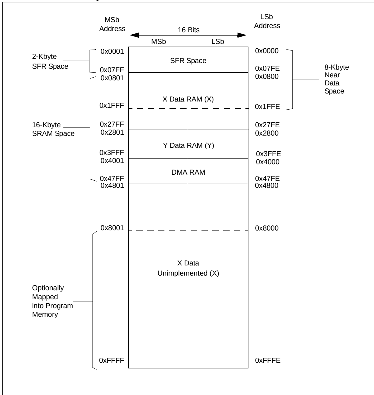
FIGURE 4-4: DATA MEMORY MAP FOR dsPIC33FJXXXMCX06A/X08A/X10A DEVICES WITH 16-Kbyte RAM
