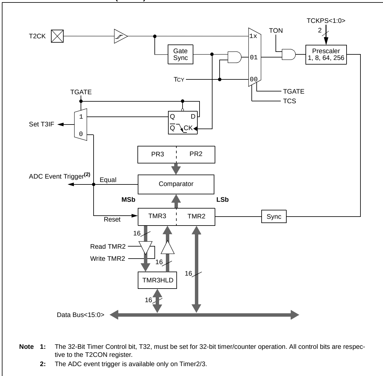
FIGURE 13-1: TIMER2/3 (32-BIT) BLOCK DIAGRAM (1)
