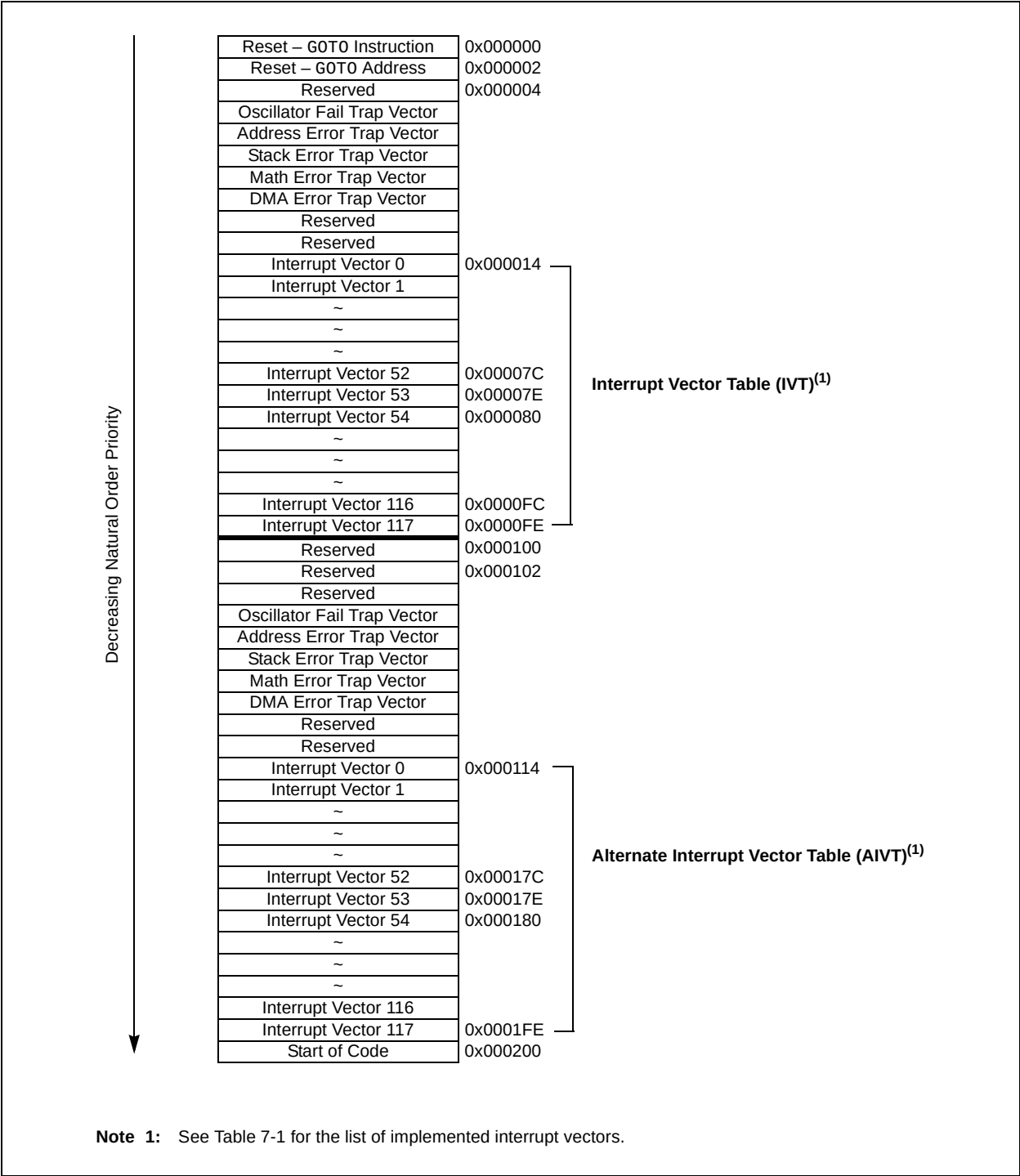
FIGURE 7-1: dsPIC33FJXXXMCX06A/X08A/X10A INTERRUPT VECTOR TABLE
