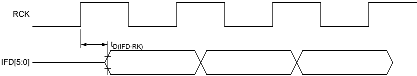
Figure 10. IFD[5:0] Bus Timing (MSEL = 1...3, Transmitting)
