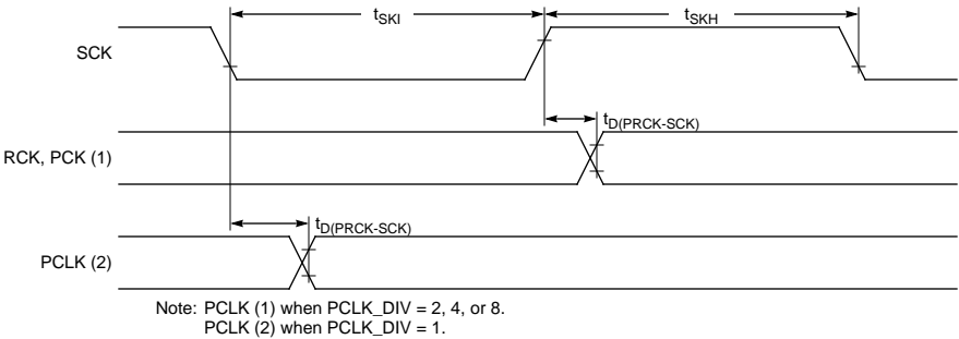
Figure 12. SCK, RCK, PCK Timing
