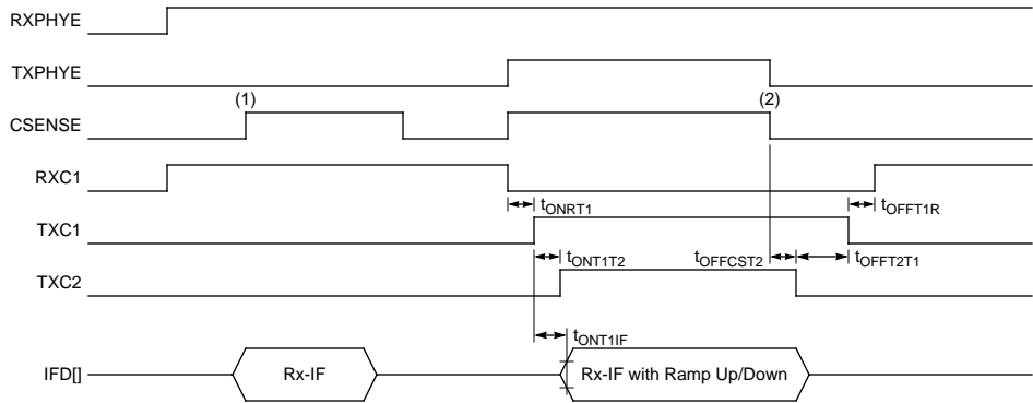
Figure 8. Radio Control Timing
