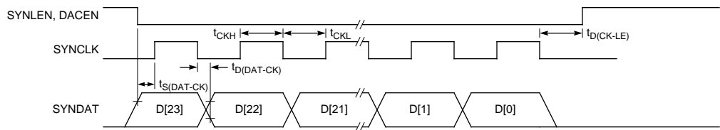
Figure 9. Synthesizer Programming Timing and DAC Timing
