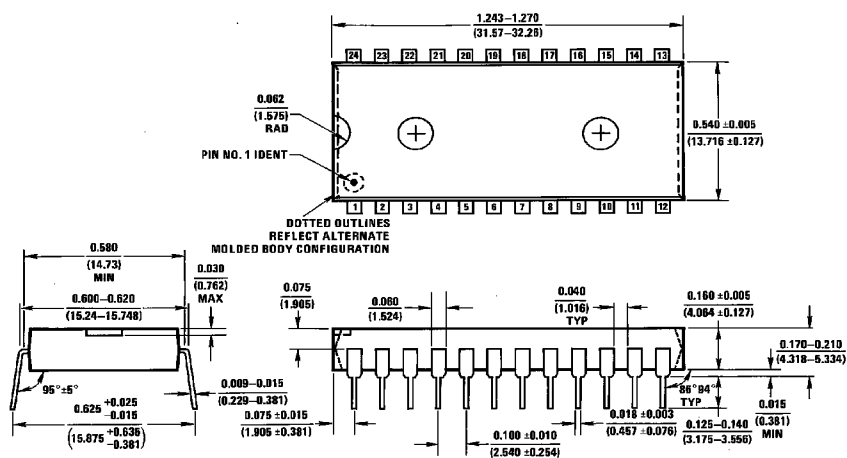
24-Lead Molded Dual-In-Line Package (N) Order Number DM74150N NS Package Number N24A
