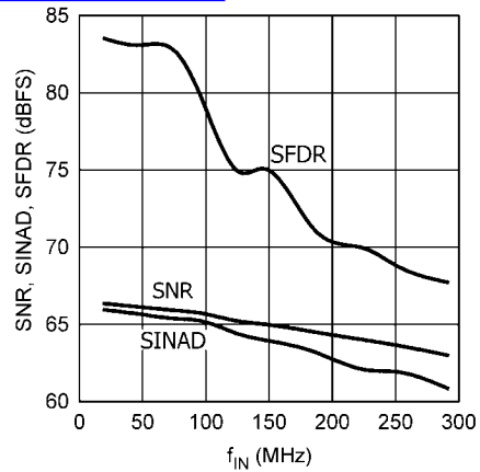
Distortion vs. f_{IN} ( f_{CLK} = 65\text{MSPS} , A_{IN} = -3\text{dBFS} )
