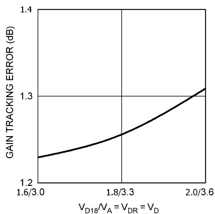
Gain Tracking Error vs. V_{SUPPLY}
