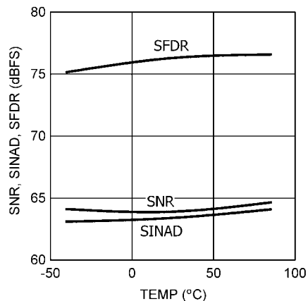
SNR, SINAD, SFDR vs. Temperature
