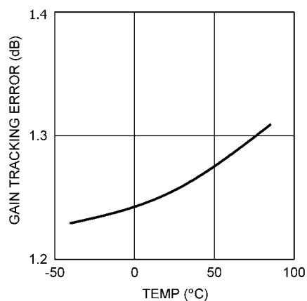
Gain Tracking Error vs. Temperature
