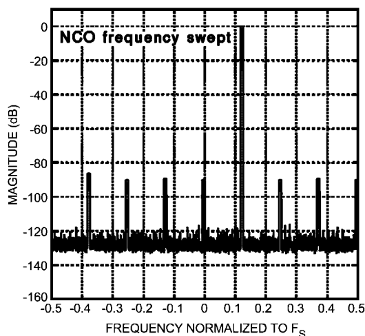
Complex NCO Output Phase Dither Disabled
