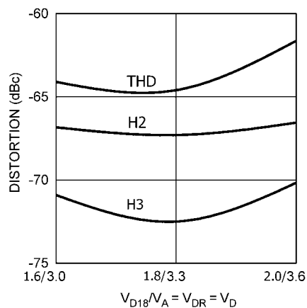
Distortion vs. V_{SUPPLY}
