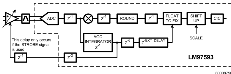
FIGURE 38. Function controlled by EXT_DELAY register
