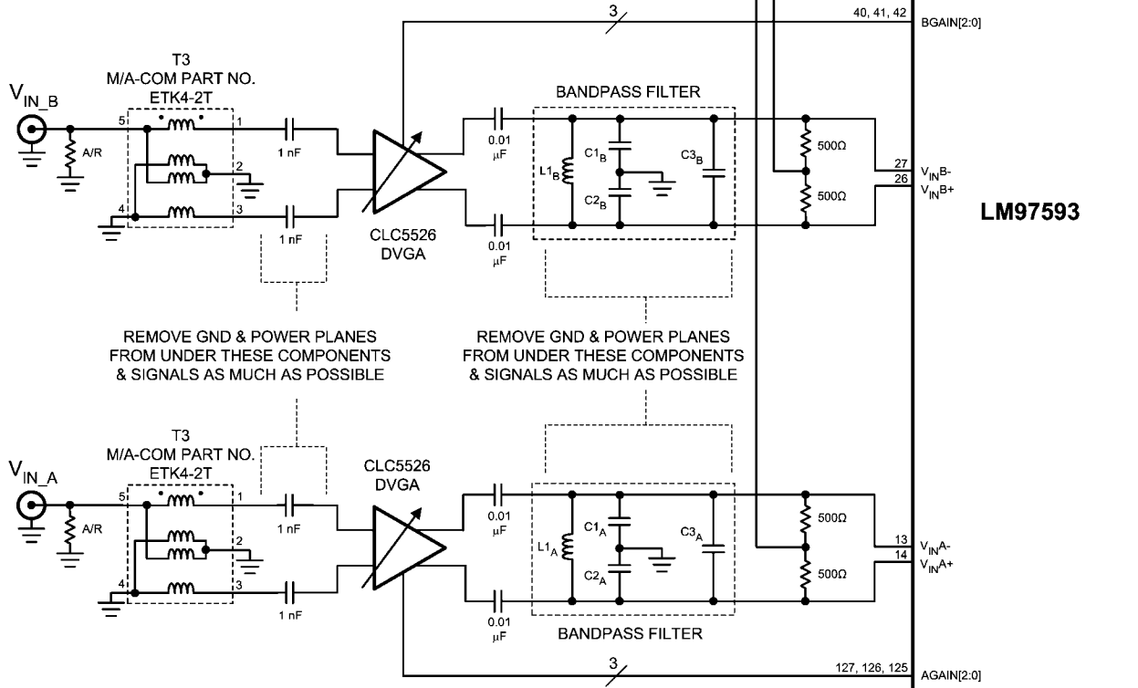
FIGURE 45. Application Circuit
