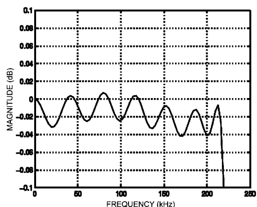
FIGURE 29. CIC, F1, &amp; F2 STD frequency response
