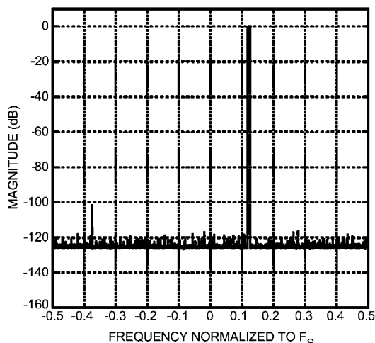
Complex NCO Output Phase Dither Enabled
