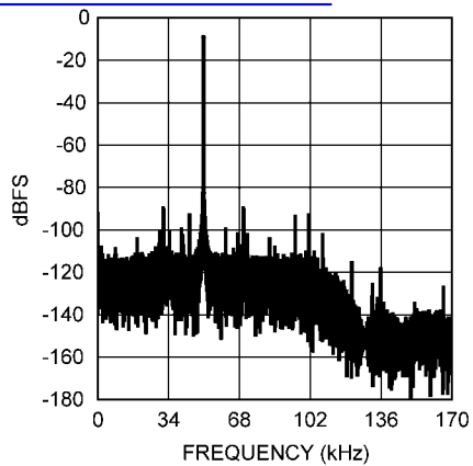
查询"LM97593"供应商 Spectral Response @ 250MHz Input ( f_{CLK} = 65\text{MSPS} , A_{IN} = -9\text{dBFS} )
