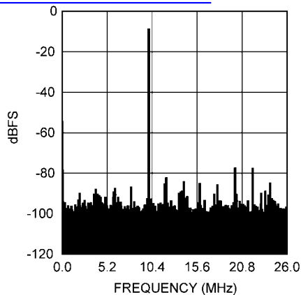
查询"LM97593"供应商 Spectral Response @ 250MHz Input ( f_{CLK} = 52MSPS , A_{IN} = -9dBFS )
