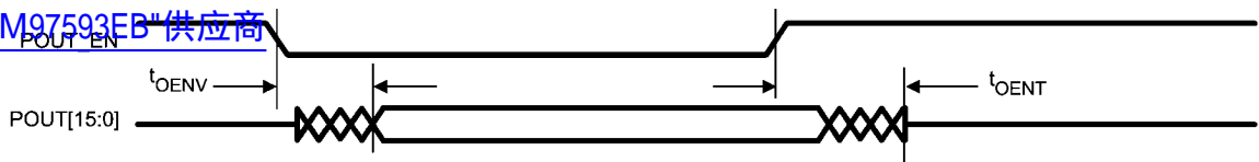
FIGURE 9. LM97593 Parallel Output Enable Timing
