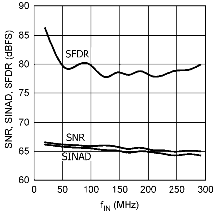
查询"LM97593"供应商 SNR, SINAD, SFDR vs. f_{IN} ( f_{CLK} = 52\text{MSPS} , A_{IN} = -9\text{dBFS} )
