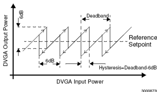
FIGURE 37. AGC Setup
