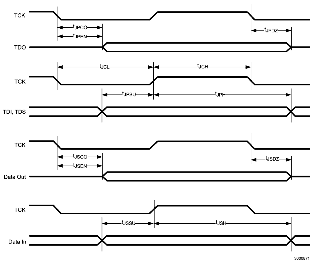
FIGURE 14. LM97593 JTAG Port Timing
