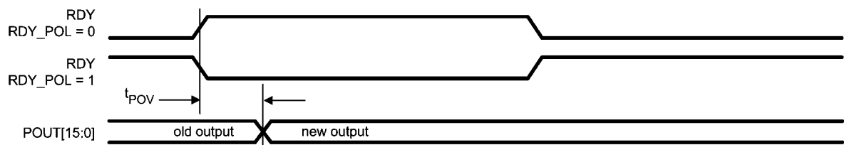
FIGURE 11. LM97593 Parallel Output Data Ready Timing
