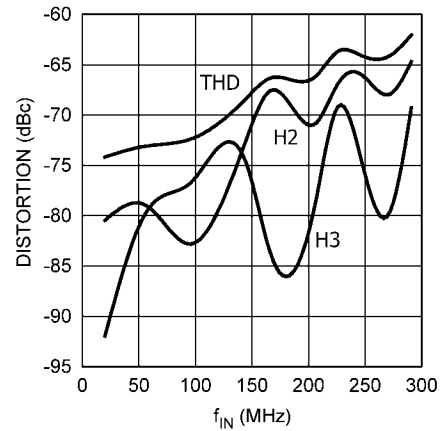
Distortion vs. f_{IN} ( f_{CLK} = 65\text{MSPS} , A_{IN} = -3\text{dBFS} )
