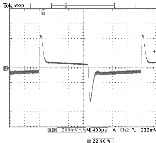
Photo 8: Transient Response Min Load to Max Load V_{in}=24V , I_{out} = 2 to 20A C_{out}=1\mu F Ceramic + 10\mu F Tantalum
