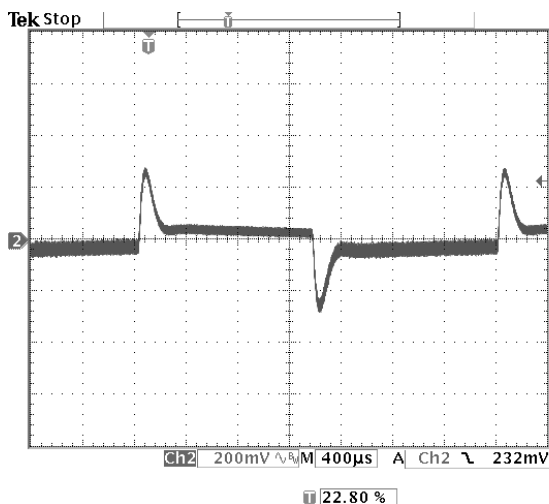
Photo 7: Transient Response 50% to 100% V_{in}=24V , I_{out} = 10 to 20A C_{out}=1\mu F Ceramic + 10\mu F Tantalum
