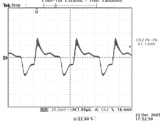
Photo 10: Output Voltage Ripple (20 MHz BW) V_{in}=24V , I_{out}=20A C_{out}=1\mu F Ceramic + 10\mu F Tantalum
