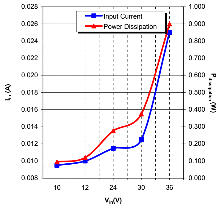
Graph 6: LV12S5-100 "Remote Off" Input Current and Power Dissipation vs. Input Voltage
