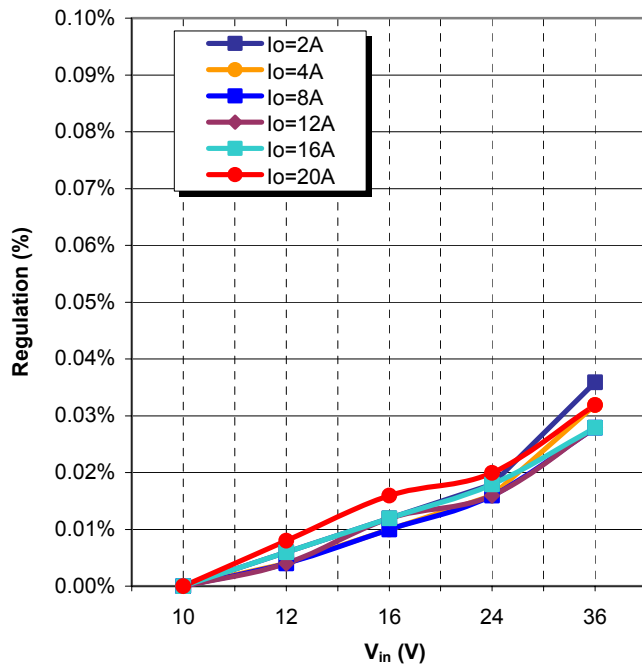
Graph 9: LV12S5-100 Line Regulation ( \pm RS Pins Open)
