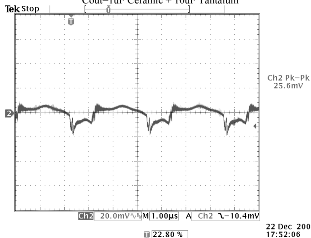
Photo 9: Output Voltage Ripple (20 MHz BW) V_{in}=24V , I_{out}=1.25A C_{out}=1\mu F Ceramic + 10\mu F Tantalum
