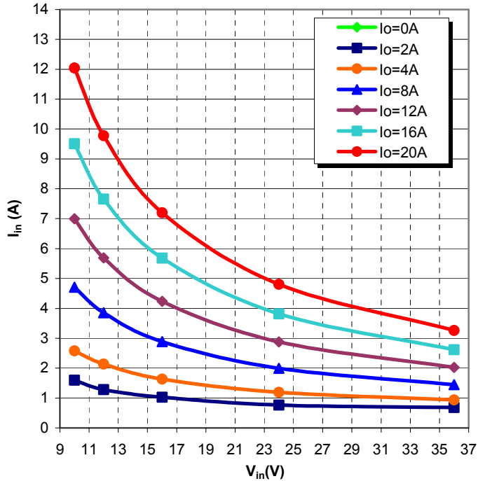
Graph 3: LV12S5-100 Input Current vs. Input Voltage
