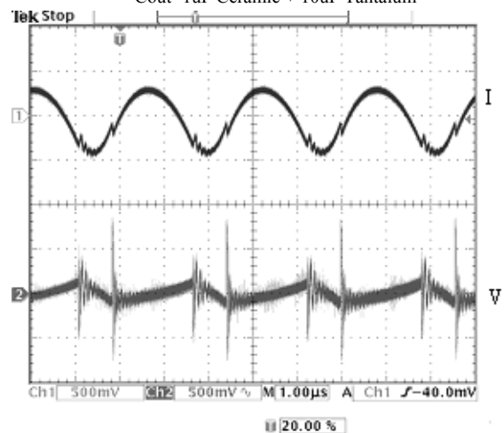
Photo 12: Input Reflected Ripple Voltage and Ripple Current V_{in}=24V , I_{out} = 20A with a 680\mu F Aluminum Electrolytic and 12\mu H series inductor.
