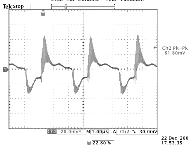
Photo 11: Output Voltage Ripple (Spike) V_{in}=24V , I_{out} = 20A C_{out}=1\mu F Ceramic + 10\mu F Tantalum
