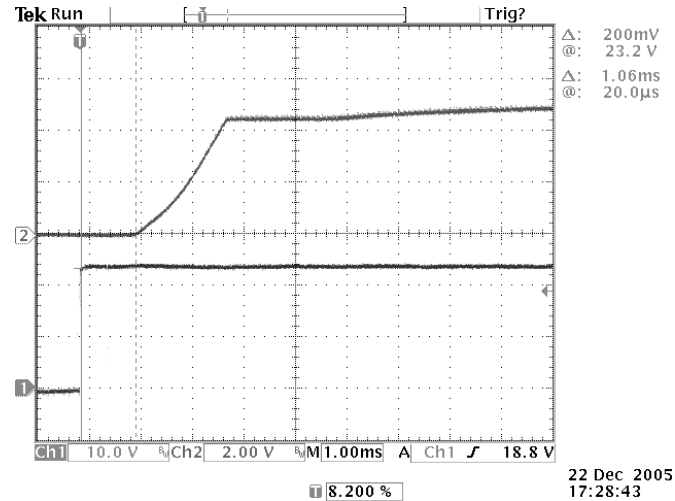
Photo 2: Remote Turn On Vin=24V, Iout = 20A,
