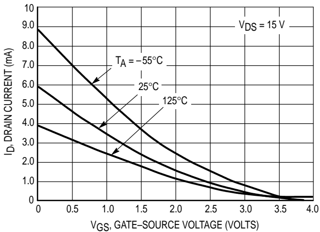
Figure 2. V_{GS(off)} = 4.0 Volts
