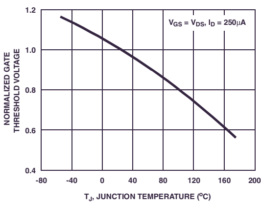
Figure 11. Normalized Gate Threshold Voltage vs Junction Temperature
