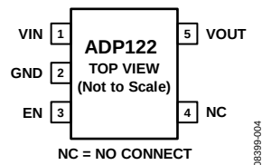
Figure 3. ADP122 Fixed Output Pin Configuration
