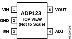
Figure 4. ADP123 Adjustable Output Pin Configuration
