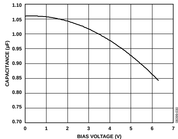
Figure 30. Capacitance vs. Capacitor Voltage Bias Characteristics
