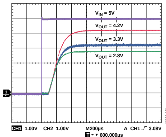
Figure 33. Typical Start-Up Time
