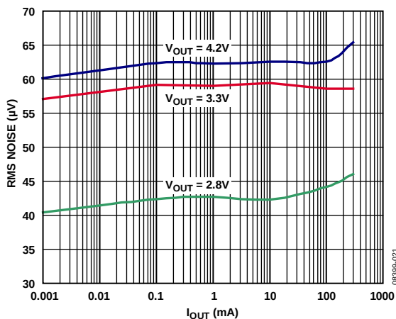
Figure 21 Output Noise vs. Load Current and Output Voltage
