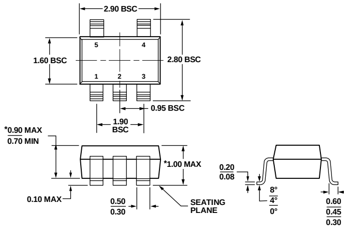
*COMPLIANT TO JEDEC STANDARDS MO-193-AB WITH THE EXCEPTION OF PACKAGE HEIGHT AND THICKNESS. Figure 43. 5-Lead Thin Small Outline Transistor Package [TSOT] (UJ-5) Dimensions shown in millimeters
