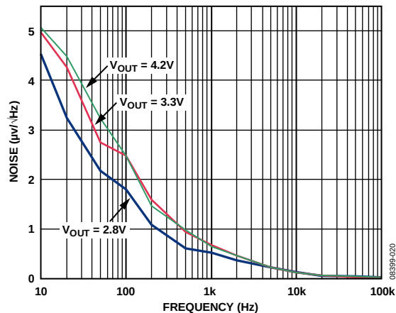
Figure 20. Output Noise Spectrum
