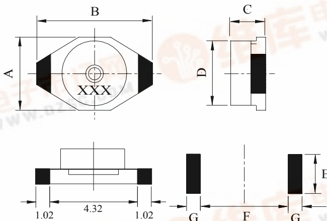
Land Pattern
