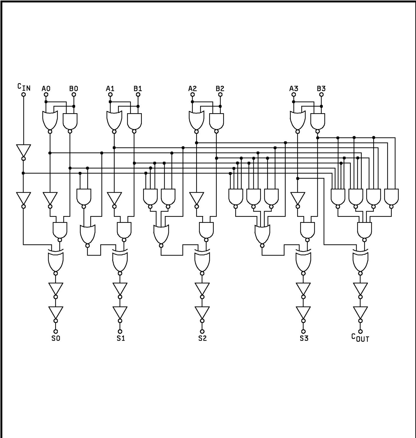
FIGURE 3. Logic diagram.
