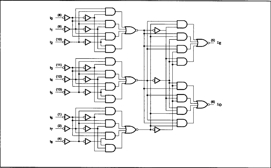
LOGIC DIAGRAM
