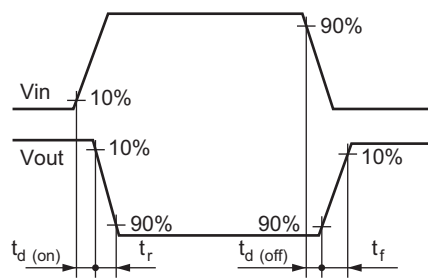
Waveforms
