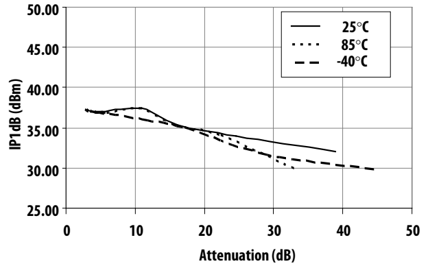
Figure 29. Input P1dB vs Attenuation vs Temperature at 1900MHz
