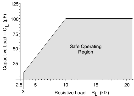
Figure 3. Maximum Loading
