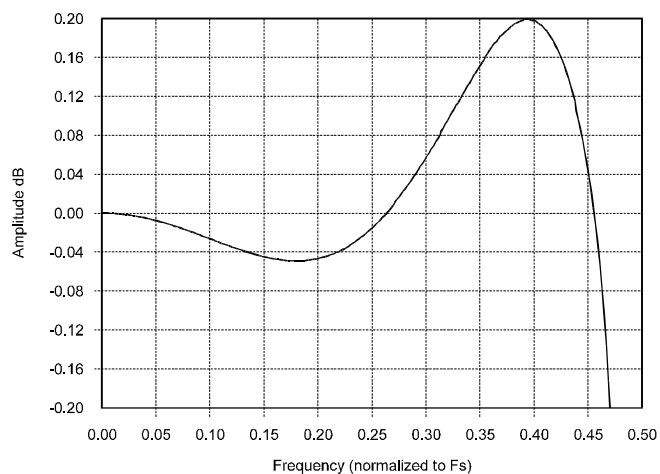
Figure 11. Double-speed Passband Ripple
