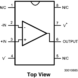
8-Pin SOIC (LMP7717)
