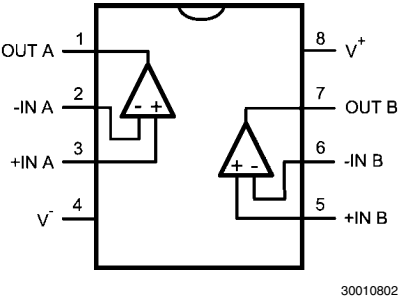
8-Pin SOIC/MSOP (LMP7718)
