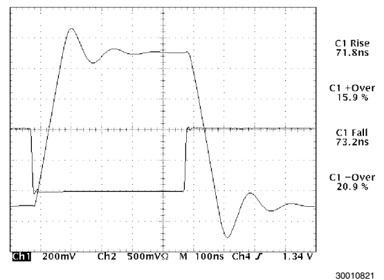
FIGURE 10. LMP7715 Response
