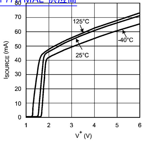
查询"LMP7717MAE"供应商 Sourcing Current vs. Supply Voltage
