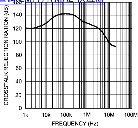
Crosstalk Rejection 查询"LMP7717MAE"供应商
