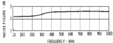
Noise Figure
