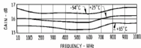
Gain
