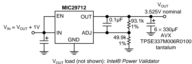
MIC29712 Load Transient Response Test Circuit
