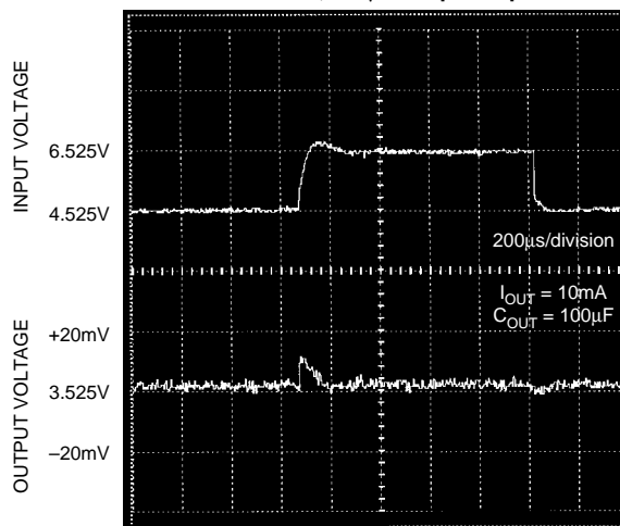
MIC29712 Line Transient Response with 10mA Load, 100 \mu F Output Capacitance
