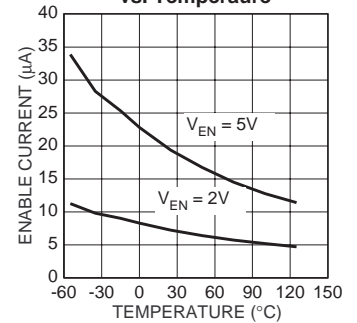
MIC29712 Enable Current vs. Temperature
