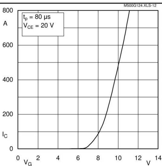
Fig. 5 Typ. transfer characteristic
