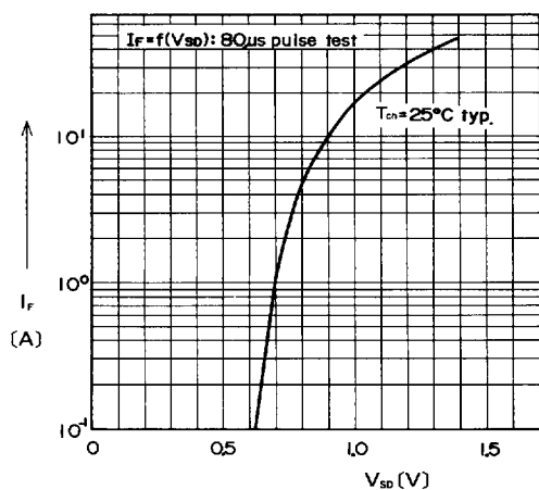
Forward Characteristic of Reverse Diode
