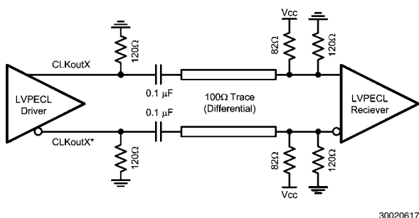
FIGURE 8. Differential LVPECL Operation, AC Coupling, Thevenin Equivalent
