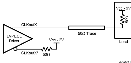
FIGURE 9. Single-Ended LVPECL Operation, DC Coupling
