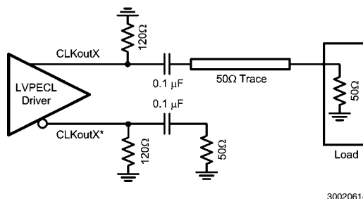
FIGURE 11. Single-Ended LVPECL Operation, AC Coupling
