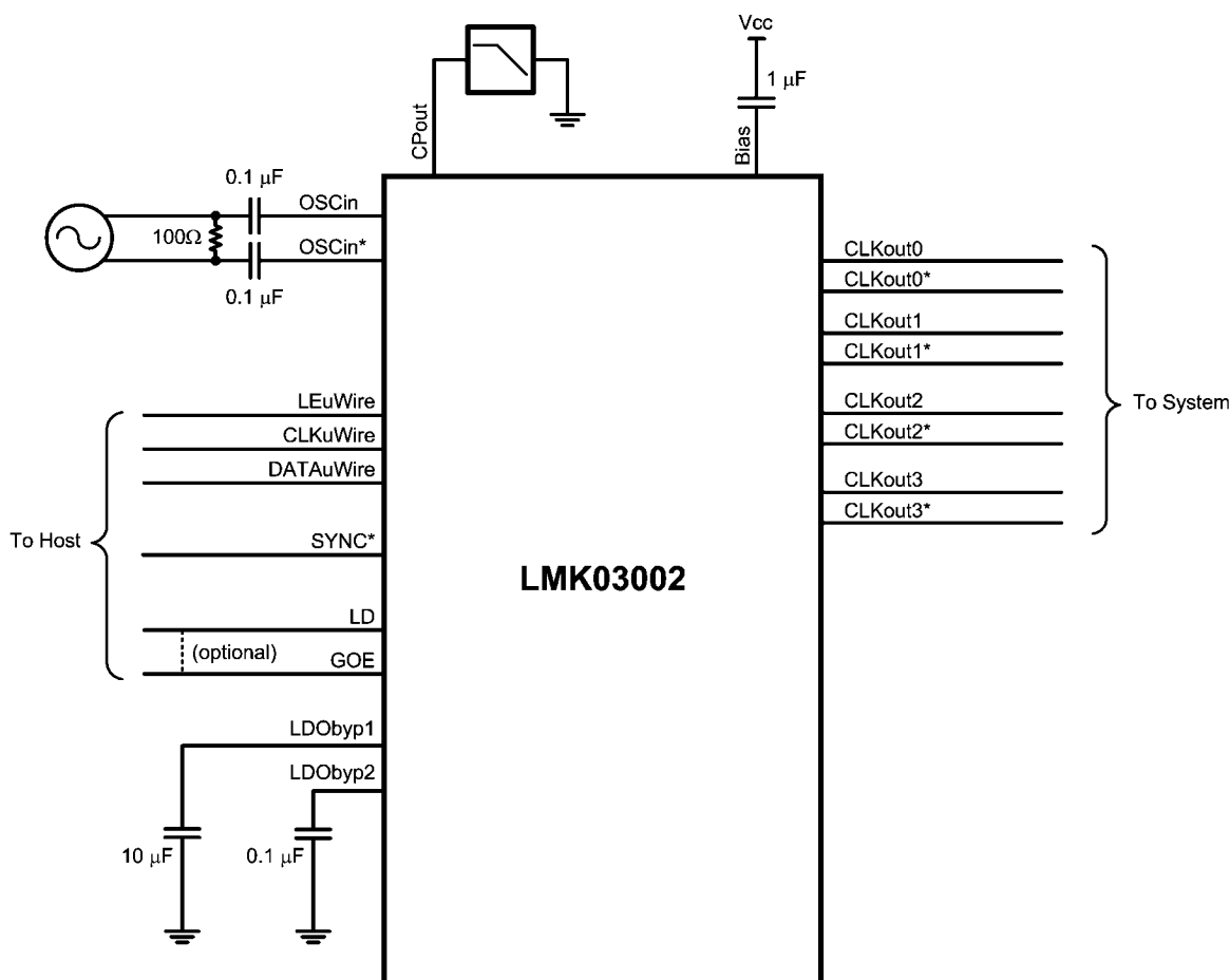
FIGURE 3. Typical Application
