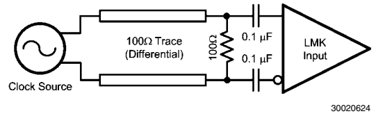
FIGURE 13. Differential Sine Wave Input
