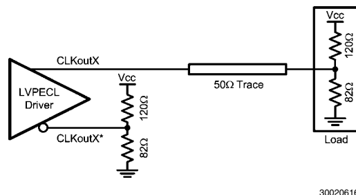
FIGURE 10. Single-Ended LVPECL Operation, DC Coupling, Thevenin Equivalent
