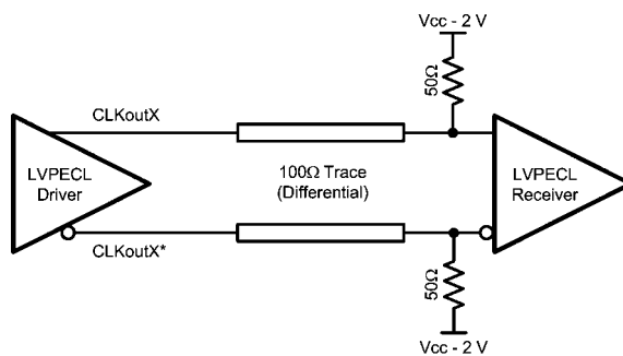
FIGURE 6. Differential LVPECL Operation, DC Coupling
