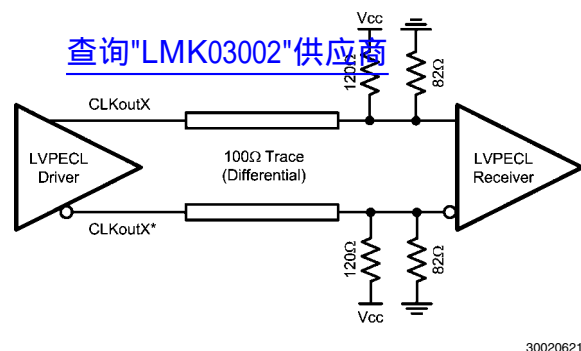
FIGURE 7. Differential LVPECL Operation, DC Coupling, Thevenin Equivalent
