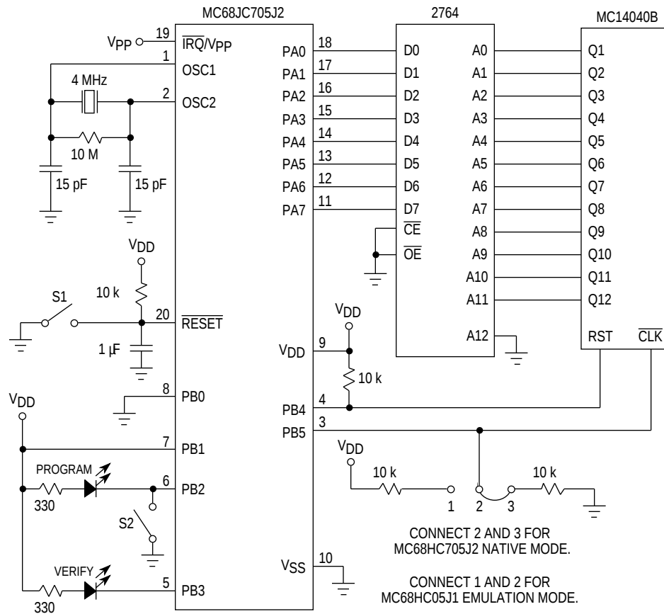
Figure 8-1. Bootloader Circuit
