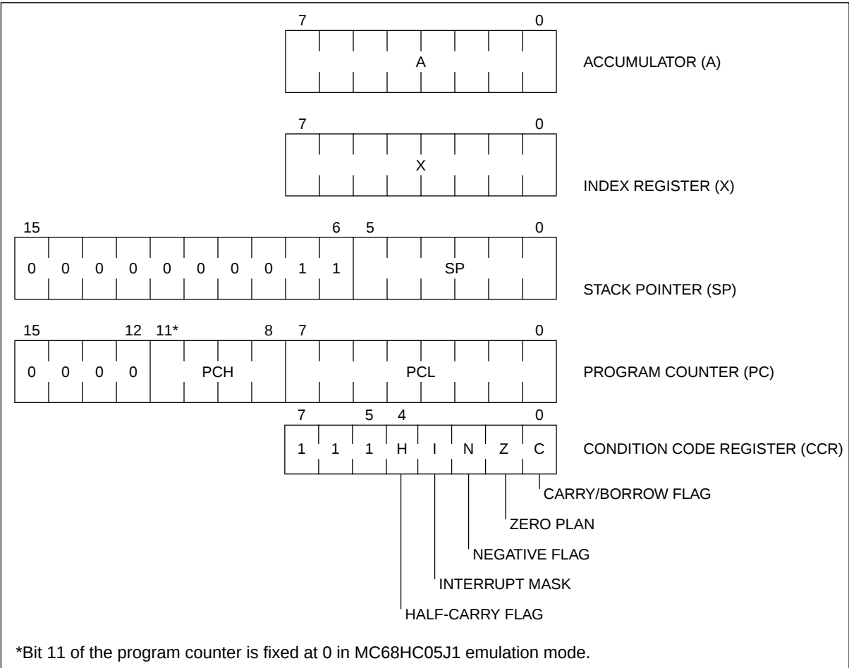
Figure 4-1. Programming Model
