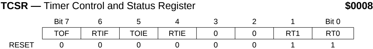
Figure 7-3. Timer Control and Status Register (TCSR)
