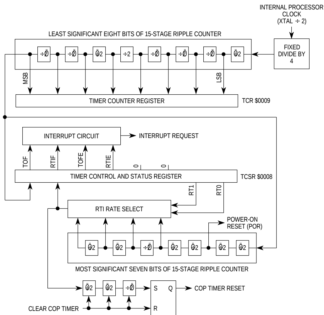
Figure 7-1. Timer
