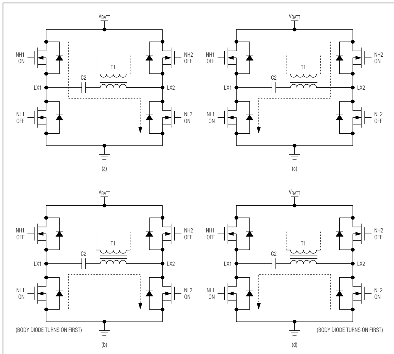
Figure 3. Resonant Operation
