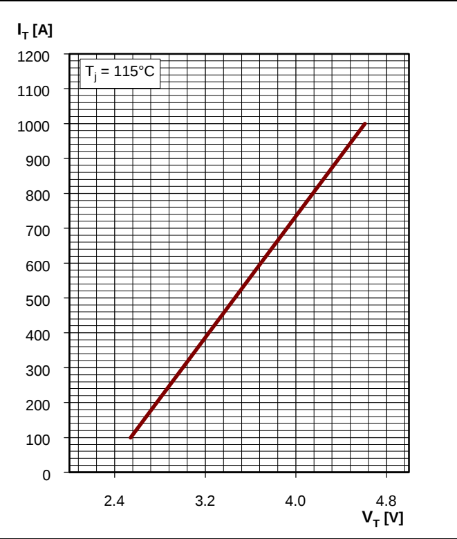
Fig. 3 GCT on-state voltage characteristics
