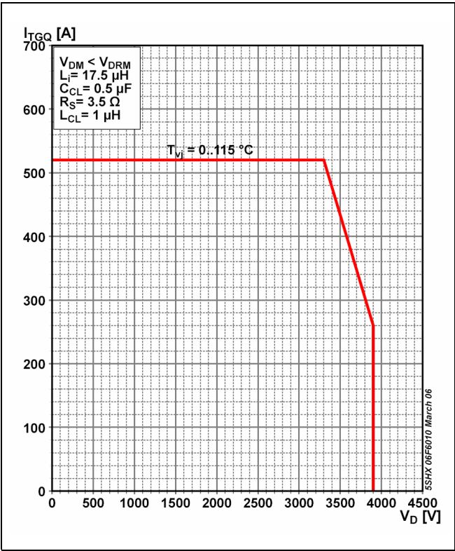
Fig. 8 GCT Safe Operating Area
