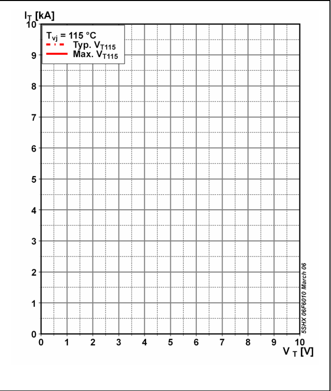
Fig. 4 GCT on-state voltage characteristics
