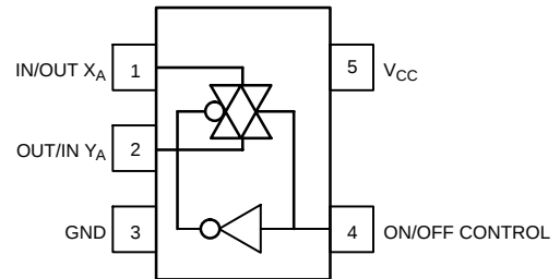
Figure 1. Pinout
