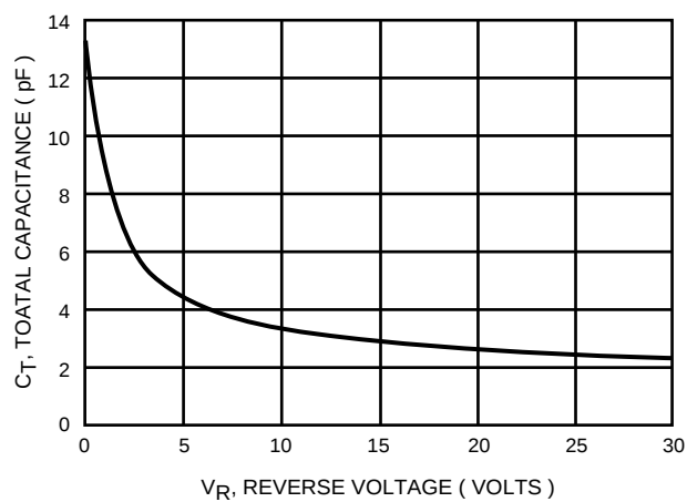
FIGURE 4. TOTAL CAPACITANCE
