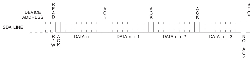
Figure 6. Sequential Read
