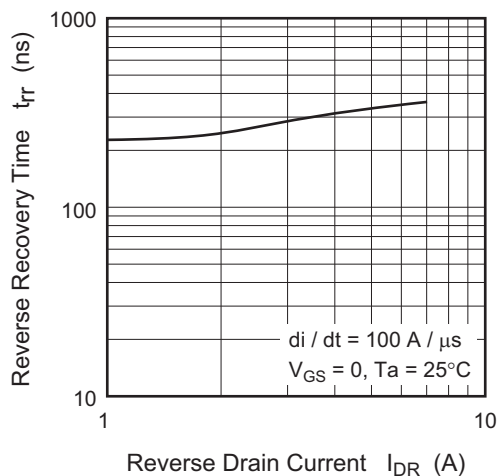
Body-Diode Reverse Recovery Time (Typical)
