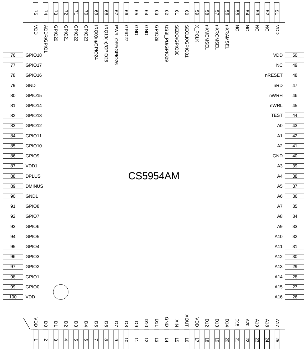
Figure 6-1. 100-pin PQFP
