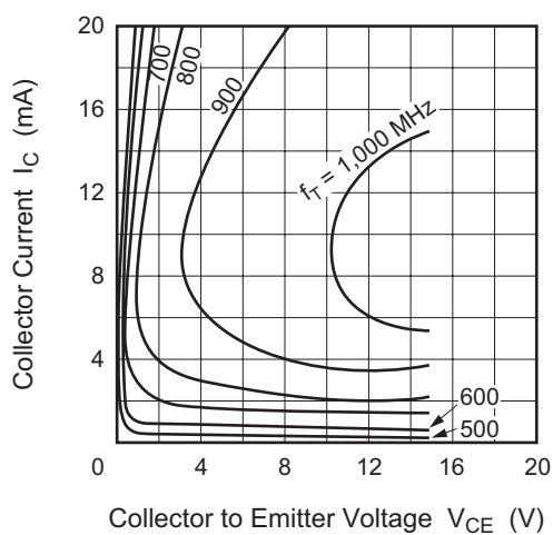
Gain Bandwidth Product Curve
