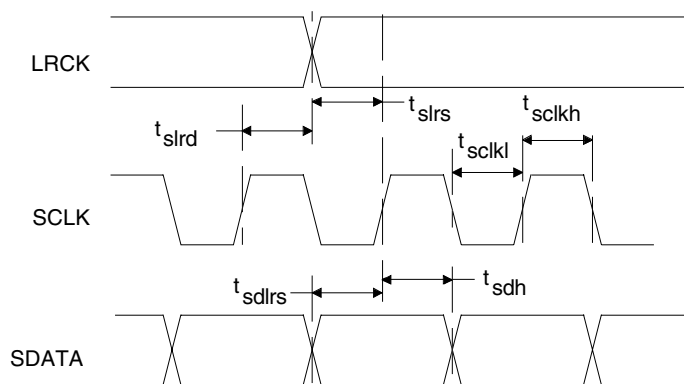
Figure 4. External Serial Mode Input Timing
