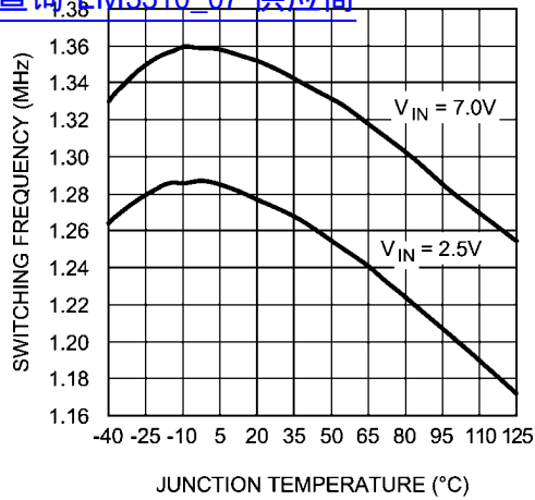
1.28MHz Switching Frequency vs. Temperature
