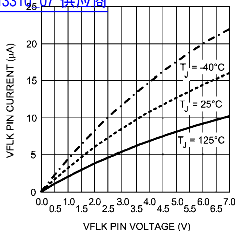
VFLK Pin Current vs. VFLK Pin Voltage
