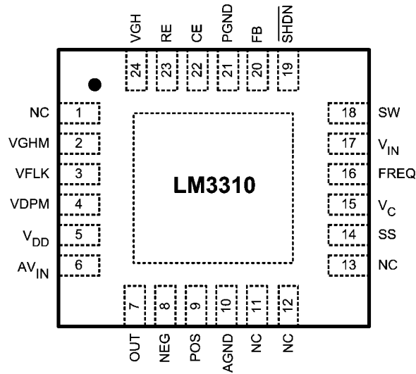
LLP-24 (Top View)
