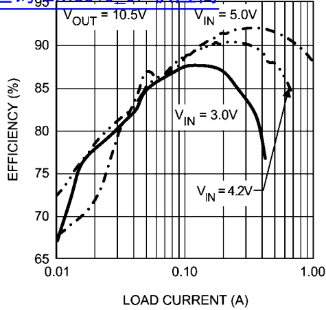
1.28MHz Application Efficiency 查询"LM3310_07"供应商
