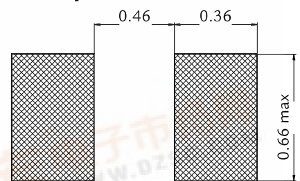
Pad layout
