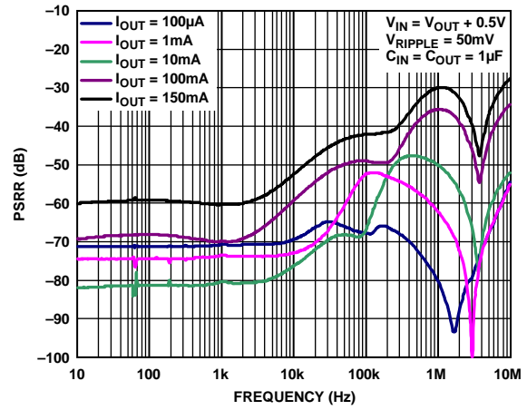
Figure 15. Power Supply Rejection Ratio (PSRR) vs. Frequency, V_{OUT} = 1.8V , V_{IN} = 2.3V
