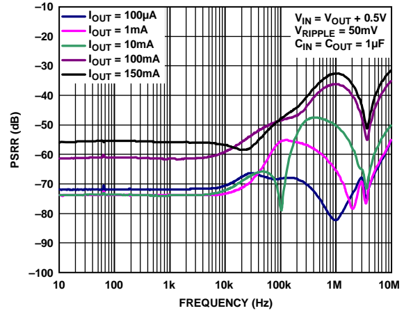
Figure 16. Power Supply Rejection Ratio (PSRR) vs. Frequency, V_{OUT} = 2.8V , V_{IN} = 3.3V
