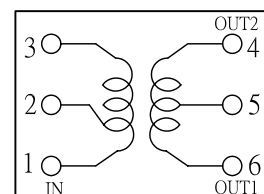
Distributor Fig.4
