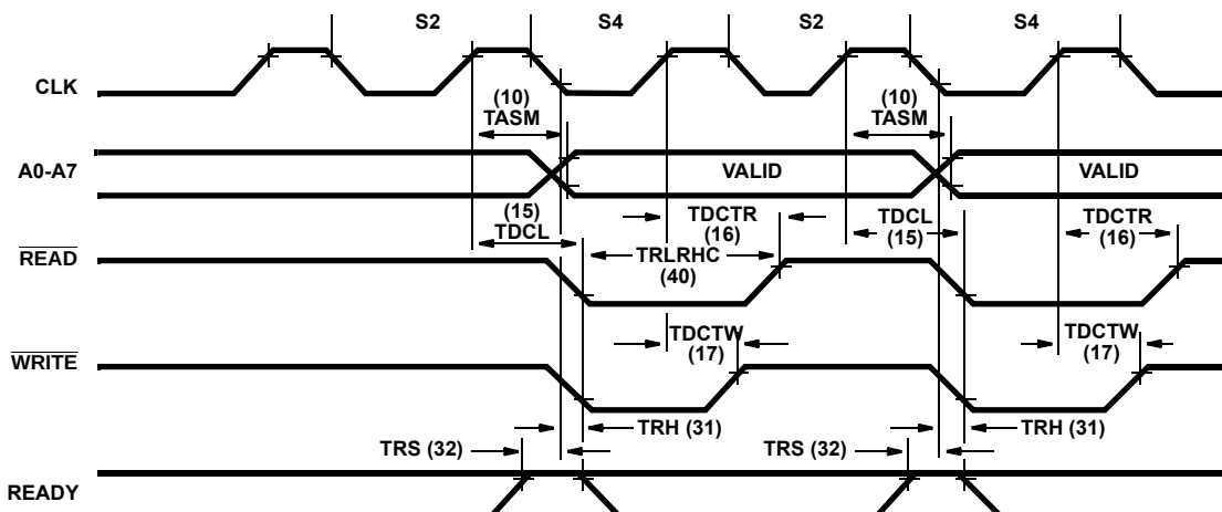
FIGURE 13. COMPRESSED TRANSFER
