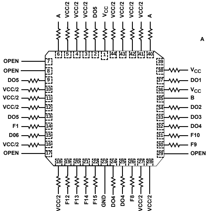
MR82C37A CLCC
