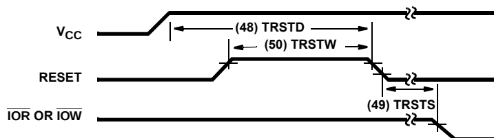
FIGURE 14. RESET
