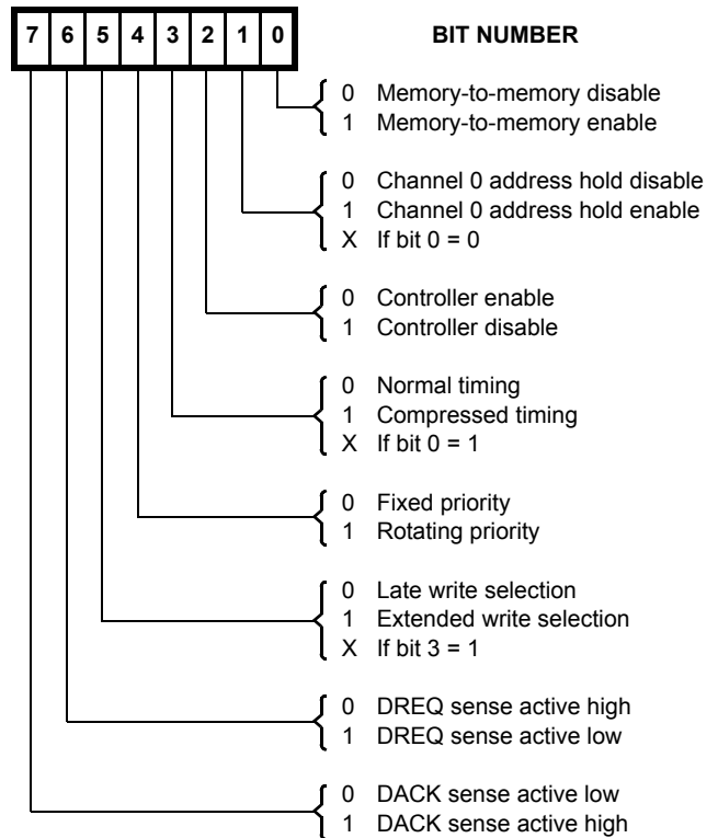
Command Register
