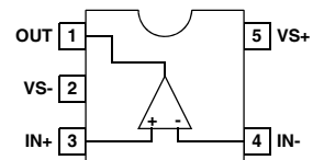
EL5193 (5 LD SOT-23) TOP VIEW
