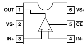
EL5193A (6 LD SOT-23) TOP VIEW
