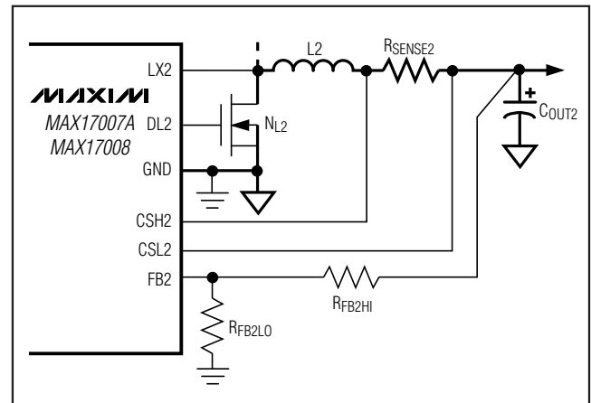
Figure 10. Setting V_{OUT2} with a Resistive Voltage-Divider
