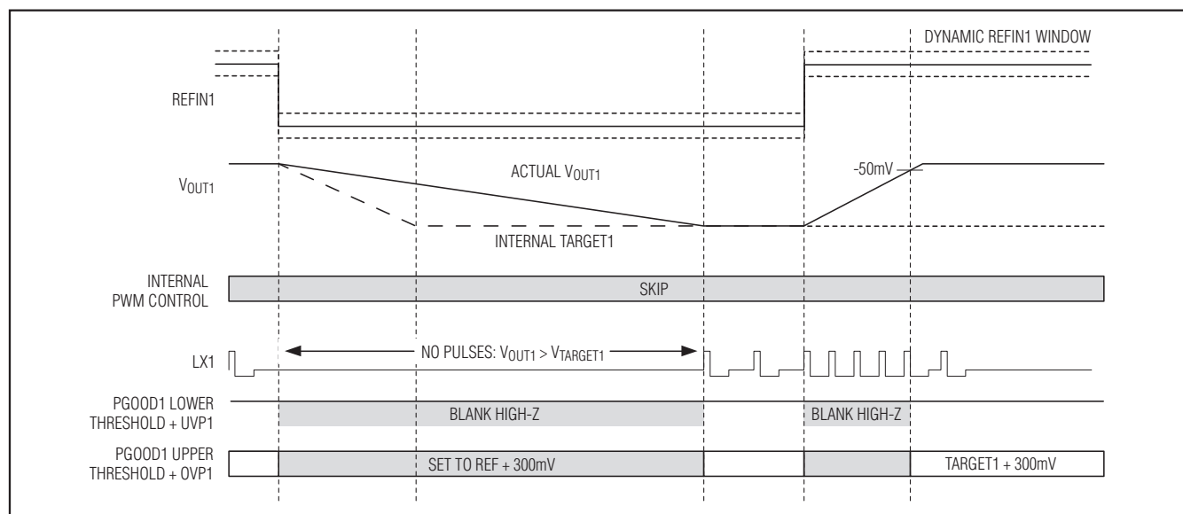
Figure 11. Dynamic REFIN1 Transition (SKIP = GND)
