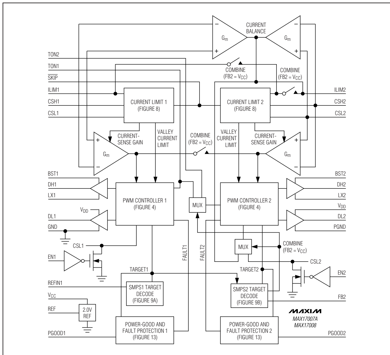
Figure 3. MAX17007A/MAX17008 Functional Diagram
