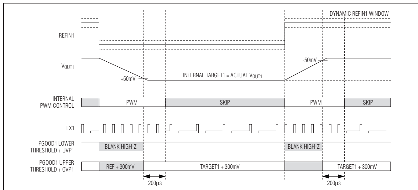
Figure 12. Dynamic REFIN1 Transition (SKIP = REF)
