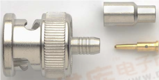
Model 7040 BNC (M) 50 \Omega Crimp
