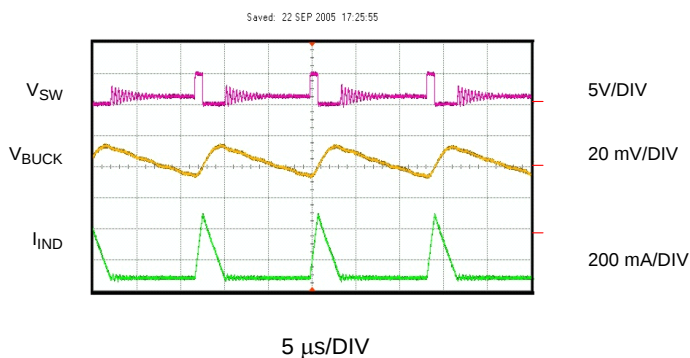
Figure 25: Switching Waveforms - DCM Mode
