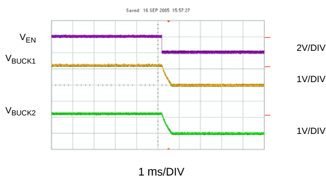
Figure 17: Turn Off Using the Enable Pin
