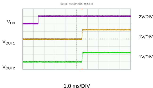
Figure 5: Startup without Sequencing
