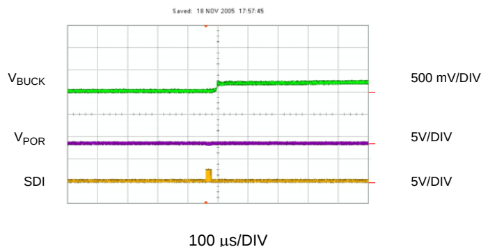
Figure 38: V_{OUT} = 1.0V to 1.2V with No Load
