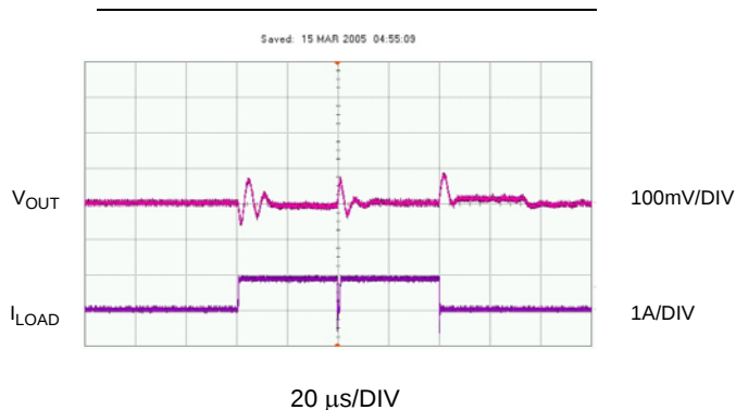
Figure 15: Adaptive Transient Response
