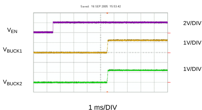
Figure 16: Startup Using the Enable Pin
