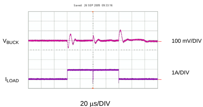
Figure 33: Double-Pulsed Load Response
