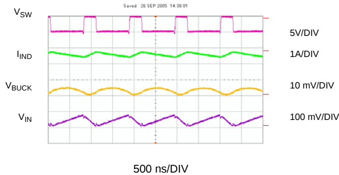
Figure 23: Switching Waveforms - PWM mode
