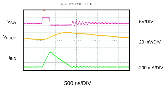
Figure 26: Switching Waveforms - DCM Mode-Zoom
