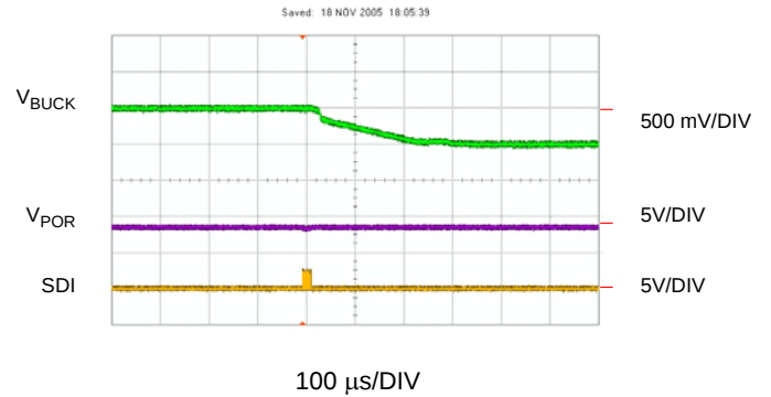
Figure 43: V_{OUT} = 1.5V to 1.0V with I_{LOAD} = 1.5A
