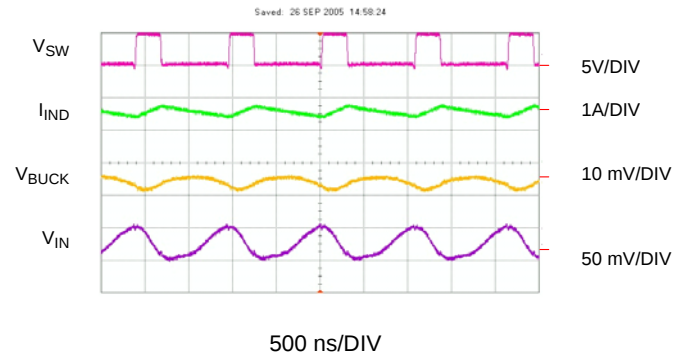
Figure 24: Switching Waveforms - PWM mode
