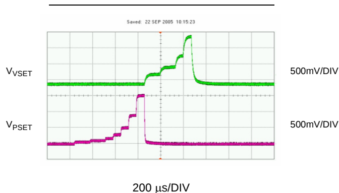
Figure 12: VSET = 2.5V and PSET = -5%
