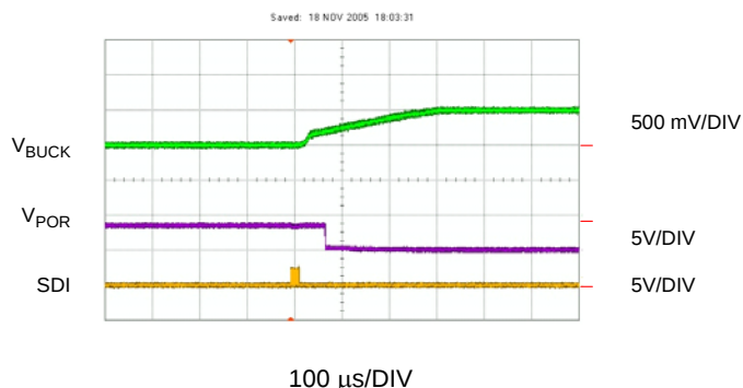
Figure 39: V_{OUT} = 1.0V to 1.5V with No Load
