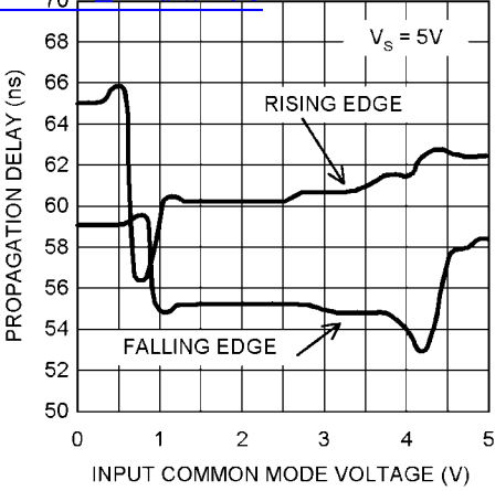
Propagation Delay vs. Common Mode Voltage 查询"LMV7235 08"供应商
