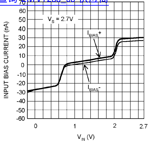
Input Bias Current vs. Input Voltage 查询"LMV7235_08"供应商
