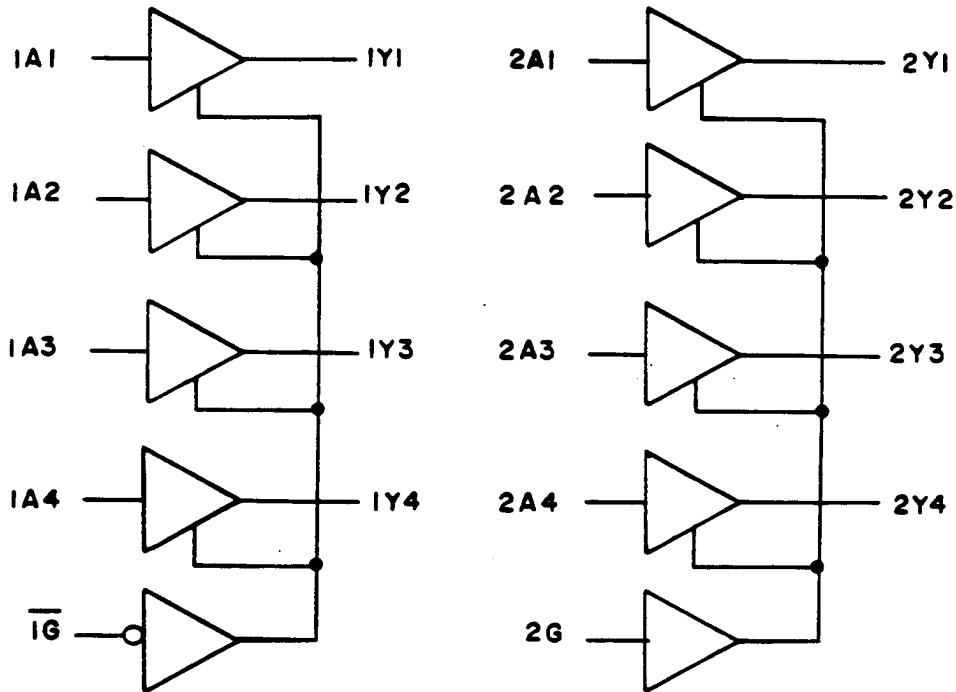
FIGURE 3. Logic diagram.
